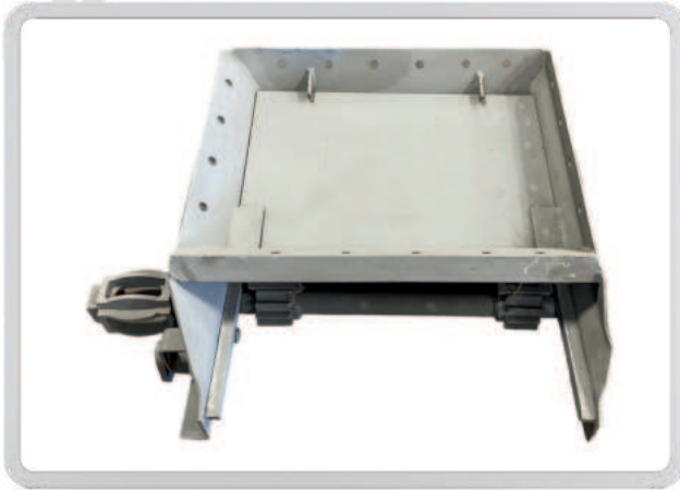
DA Pt # DA-49090 Alt Pt # DA-490-L Description: Door Gate Complete - LH
