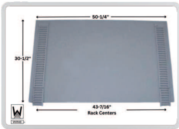
DA Pt # DA-41329 Alt Pt # 3CH-429 Description: Door Slide Assembly
