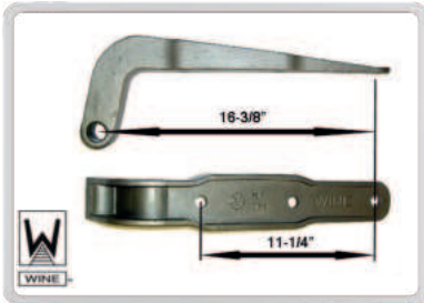
DA Pt # DA-23261 Alt Pt # HF-261 Description: Hinge, Substitutes DA-25127
