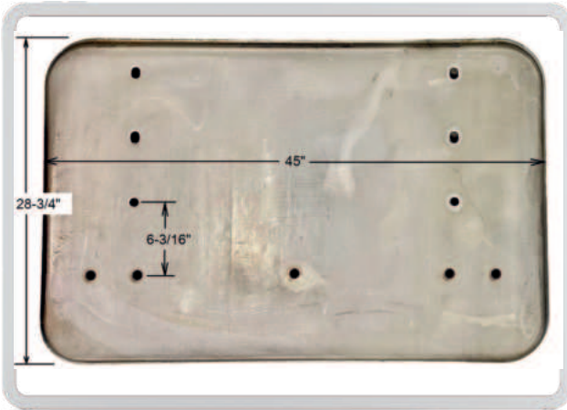
DA Pt # DA-176004-SP Alt Pt # D-170-6004 Description: Large, Carbon Steel, 5/16" Thick Hopper Door w/ Spreader Beam Holes
