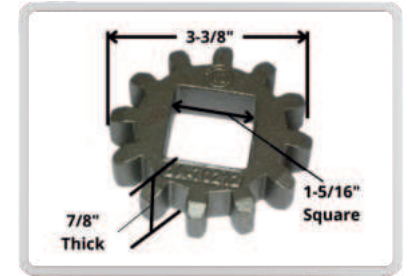
DA Pt # DA-70212 Alt Pt # 70212 Description: Pinion Gear
