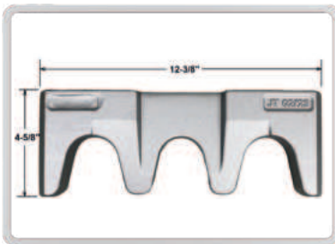
DA Pt # DA-09462 Alt Pt # 09462 Description: Draft Lug, Rear, Forging
