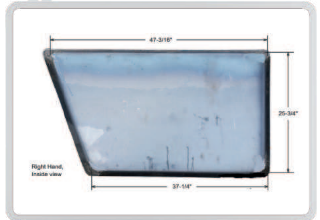
DA Pt # DA-52965 Alt Pt # 810-689671 Description: Trapezoidal, RH Hopper Door
