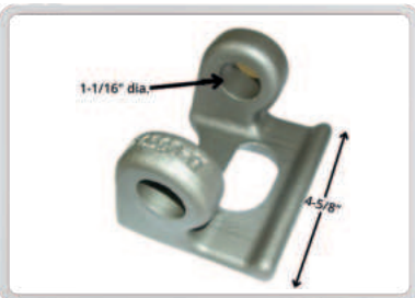
DA Pt # DA-50017 Alt Pt # 093-40020 Description: Hinge Butt
