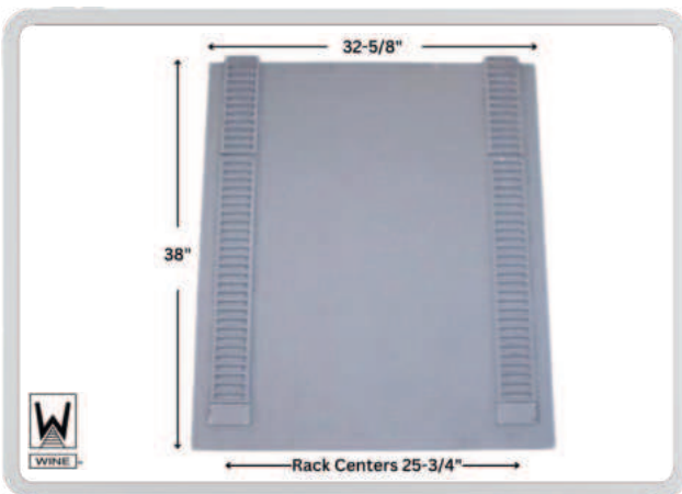
DA Pt # DA-32300 Alt Pt # 2CH-323 Description: Door Slide Assembly
