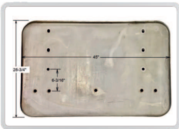
DA Pt # DA-176006-H Alt Pt # 176006H Description: Large, Carbon Steel Hopper Door, 3/8" Thick w/ Spreader holes
