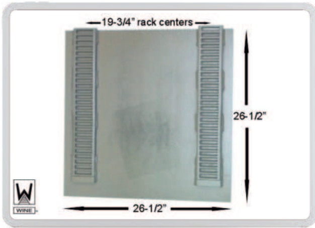
DA Pt # DA-41254 Alt Pt # 2CH-404 Description: Door Slide Assembly
