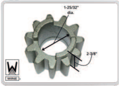
DA Pt # DA-21129 Alt Pt # 2CH-29 Description: Pinion Gear
