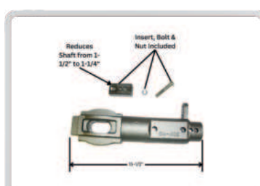
DA Pt # DA-41902 Alt Pt # DA-402 Description: Long Capstan, Universal,
