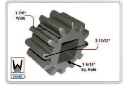
DA Pt # DA-70209 Alt Pt # DA-29-A Description: 1-7/8" Wide Pinion Gear, 1-5/16 Sq. Hole
