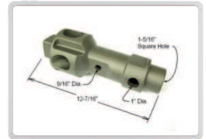
DA Pt # DA-43413 Alt Pt # DA-403 Description: Capstan
