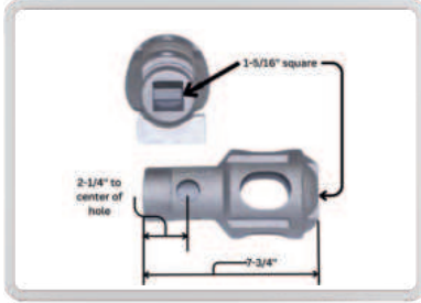
DA Pt # DA-42391 Alt Pt # DA-4081 Description: Capstan
