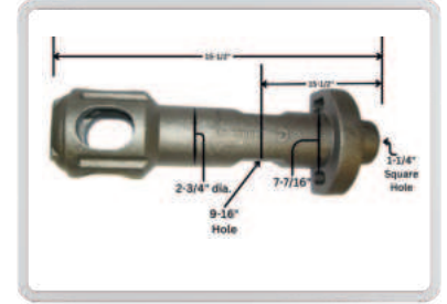
DA Pt # DA-10080 Alt Pt # 10080 Description: Capstan
