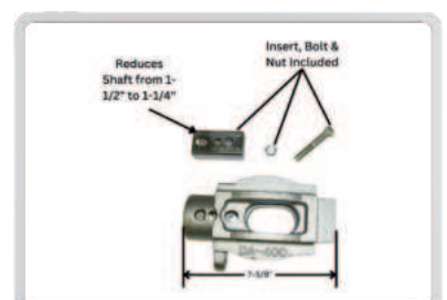
DA Pt # DA-41890 Alt Pt # DA-400 Description: Short Capstan, Universal
