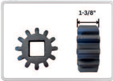
DA Pt # DA-70211 Alt Pt # 70211 Description: Pinion, 1-3/8"
