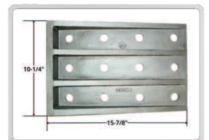
DA Pt # DA-18004 Alt Pt # B-10804 Description: Draft Lug, Rear
