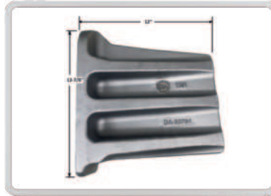
DA Pt # DA-53704 Alt Pt # 53704 Description: Draft Lug, Forging, Rear
